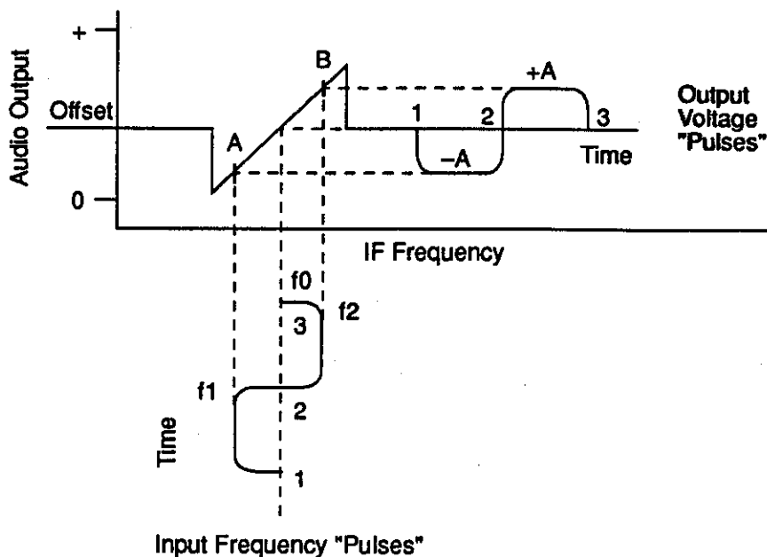
FIGURE 3. A Typical FM Detector Characteristic
